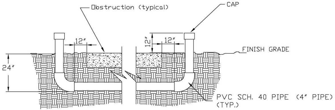
IRRIGATION SLEEVING DETAIL
