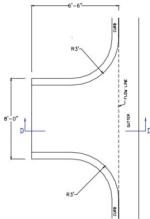
TYPICAL HANDICAP CURB CUT
