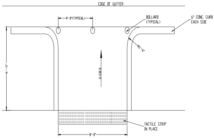
TYP. HANDICAP SIDEWALK CURB CUT
