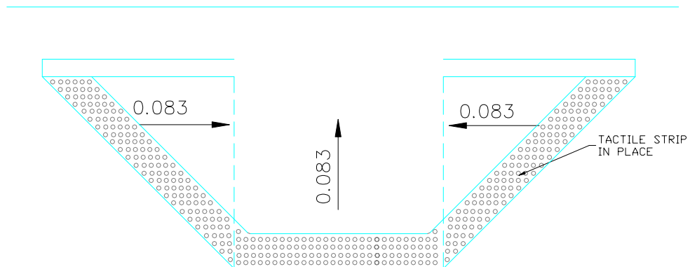
TYP. HANDICAP SIDEWALK CURB CUT NOT TO SCALE
